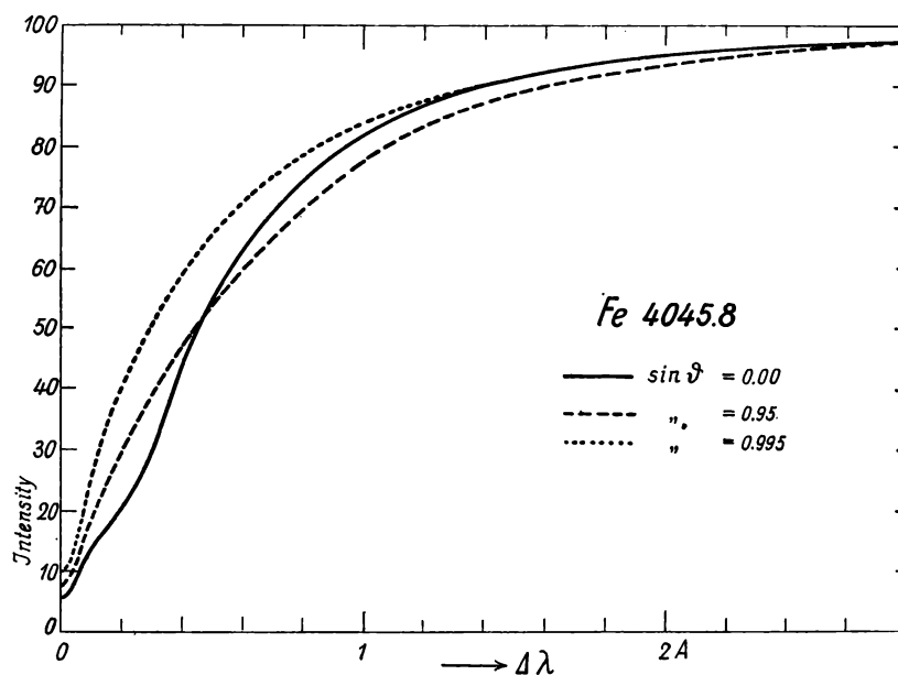
Fig. 14. — Profiles of the line Fe 4045.8 in three different points of the solar disc (non-corrected central intensities).
