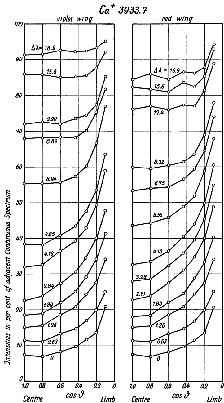
Fig. 6. — Centre-limb variations in the K line, \text{Ca}^+ 3933.7 (parameter \Delta\lambda = distance in Å from centre of line).
