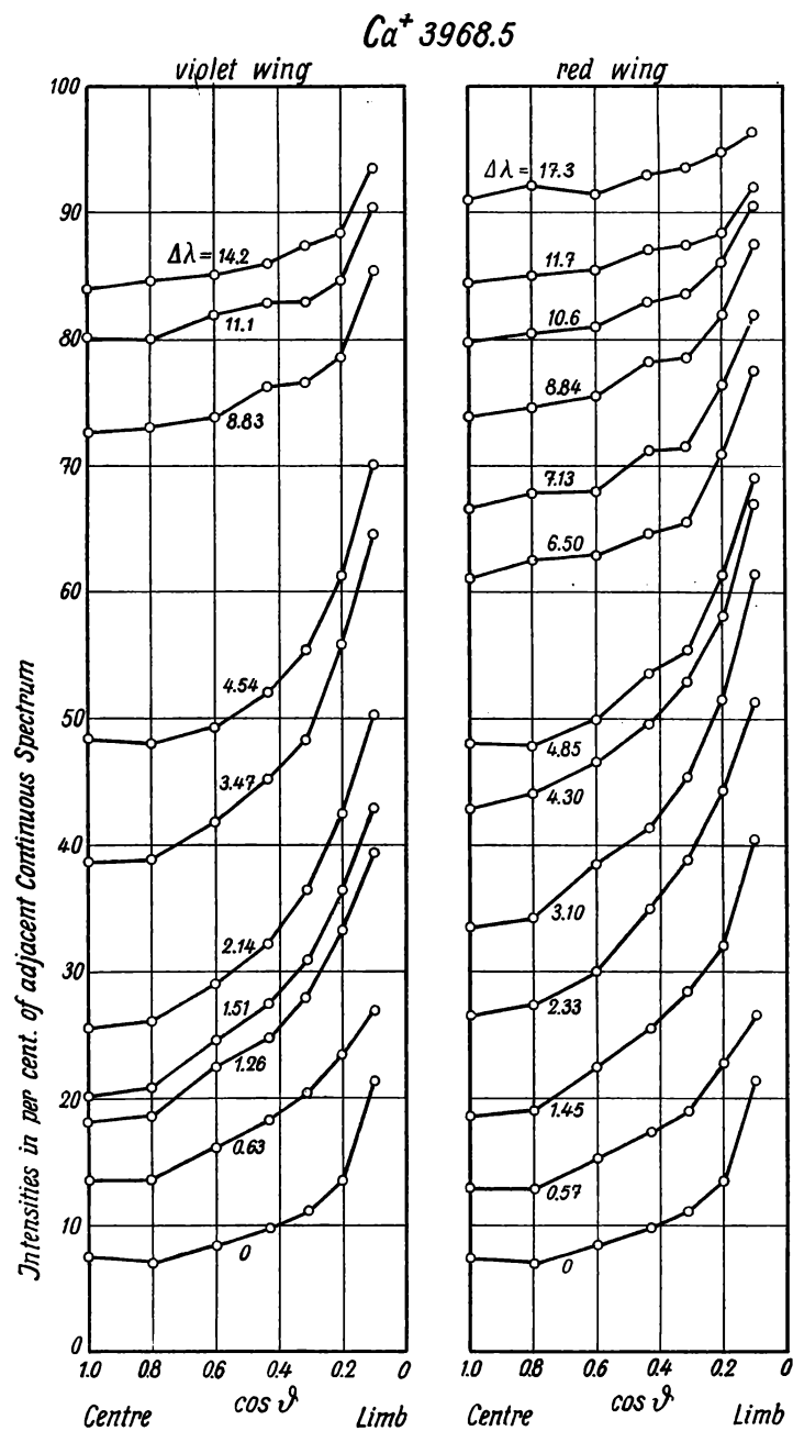
Fig. 7. — Centre-limb variations in the H line, \text{Ca}^+ 3968.5 (parameter \Delta\lambda = distance in Å from centre of line).
