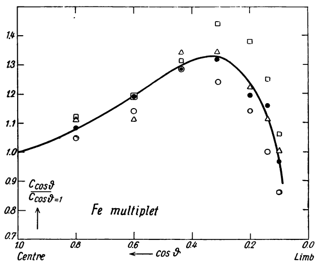
Fig. 15. — Centre-limb variations of the c 's of four lines of the Fe multiplet a^3F_4 \rightarrow \gamma^3F_3^0 ; ● Fe 4045.8; ○ Fe 4063.6; □ Fe 4071.8; △ Fe 4143.9.
