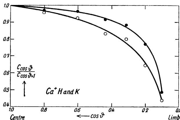
Fig. 10. — Centre-limb variations of the c 's of the H- and K line, deduced from Fig. 9; ● for the K line and ○ for the H line.
