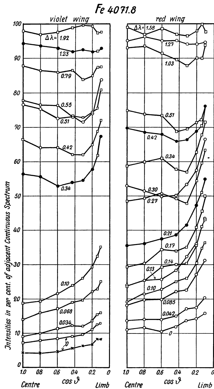
Fig. 17. — Centre-limb variations in the line Fe 4071.8; ○ Utrecht; □ Potsdam; ● mean; × corrected central intensities (parameter \Delta\lambda = distance in Å from centre of line).
