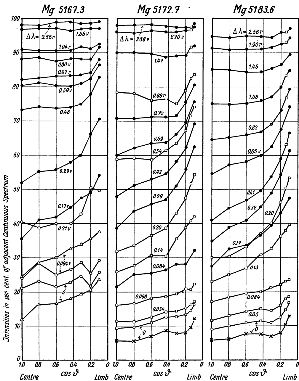
Fig. 23. — Centre-limb variations in the lines Mg 5167.3, Mg 5172.7 and Mg 5183.6; ○ Utrecht; △ Mount Wilson; □ Potsdam; ● mean of at least two of these; × corrected Potsdam central intensities (parameter \Delta\lambda = distance in Å from centre of line).
