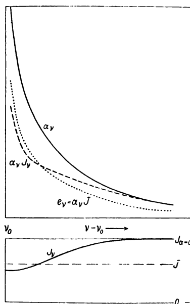
Fig. 36. Complete redistribution; absorption ( \alpha_\nu J_\nu ) and emission ( e_\nu = \alpha_\nu \bar{J} ) as functions of \nu - \nu_0 in the frequency-range of a Fraunhofer line.
