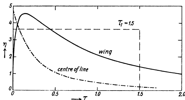
Fig. 43. — Run of \eta , the ratio of the summed up selective absorption and scattering to the continuous absorption, deduced by B. Strömgren for the Na D lines. The ordinates are expressed in arbitrary units, which differ for the wings and the centre of the line but are the same for the run in the wing and the schematic run with \tau_1 = 1.5 .
