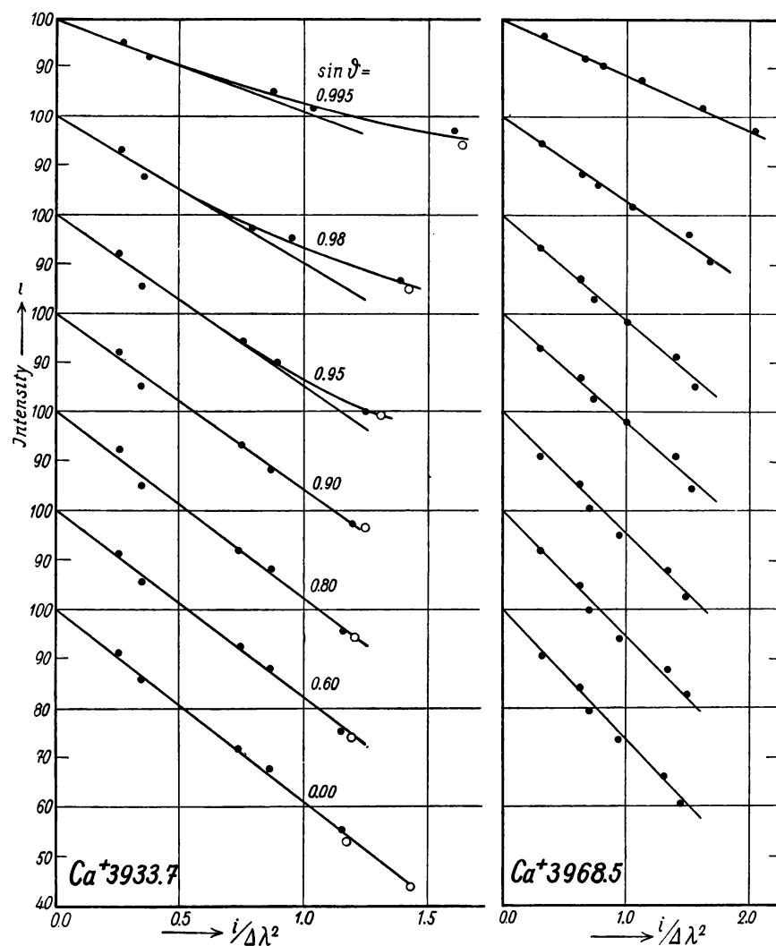
Fig. 9. — Determination of the c 's of the H- and K line of \text{Ca}^+ .
