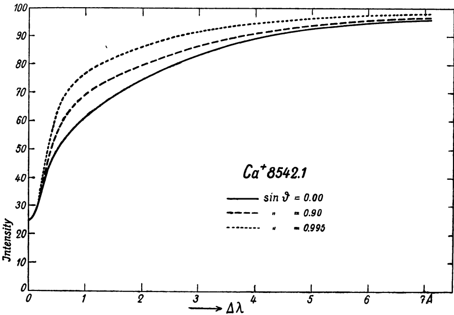
Fig. 32. — Profiles of the line \text{Ca}^+ 8542.1 in three different points of the solar disc.
