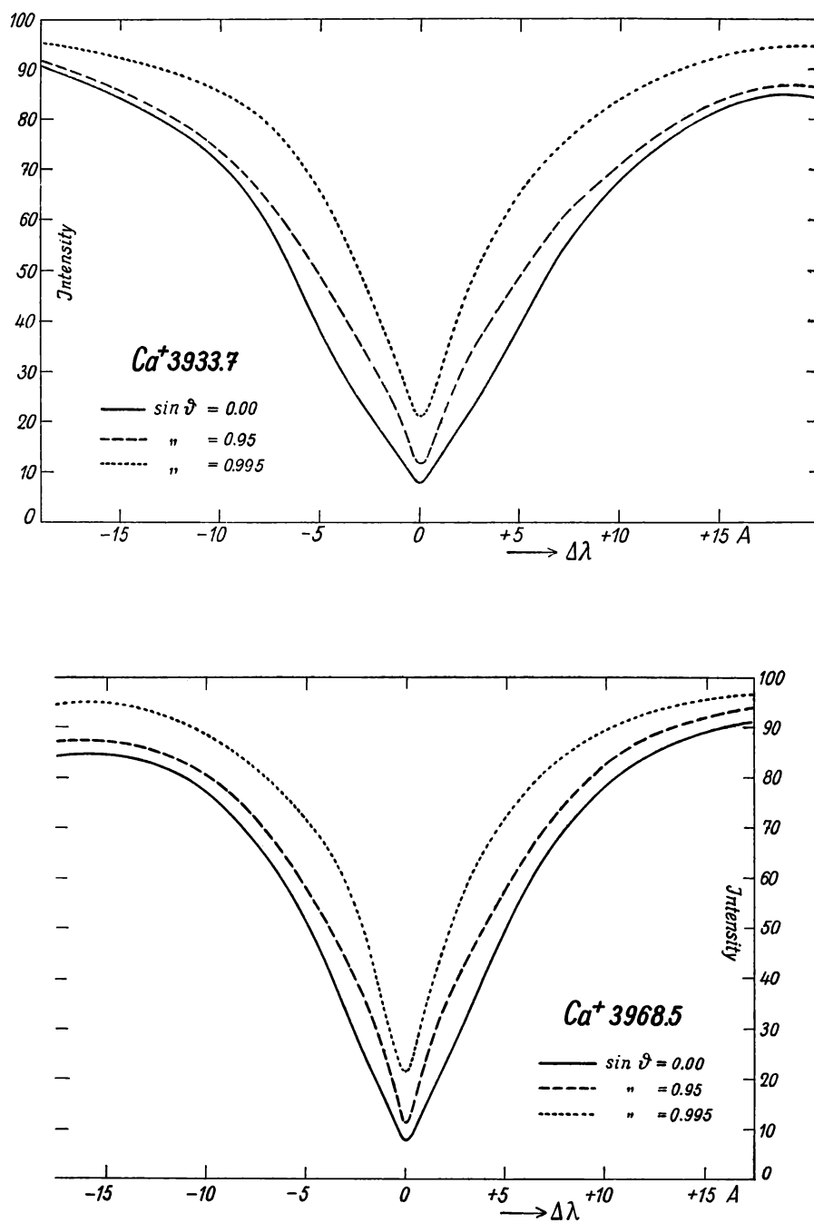
Fig. 8. — Profiles of the H line (lower fig.) and K line (upper fig.) of \text{Ca}^+ in three different points of the solar disc.
