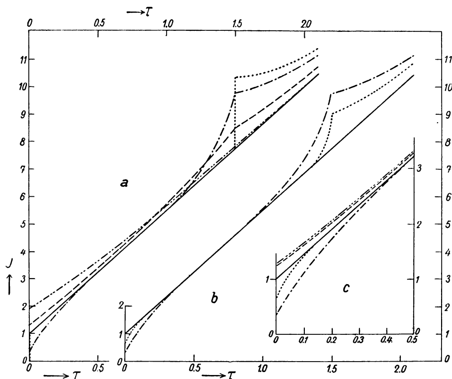
Fig. 39. — Runs of B , J(s) and J(k) with depth in the schematic model of the solar atmosphere for \beta_0 = 4.5 (all of them in terms of B_0 ).
