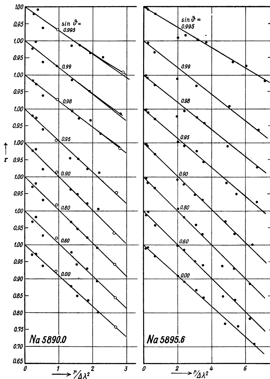
Fig. 28. — Determination of the c 's of the D lines of Na; the points \circ are the means of 3 values from the intensity lists (Tables 16 and 17).
