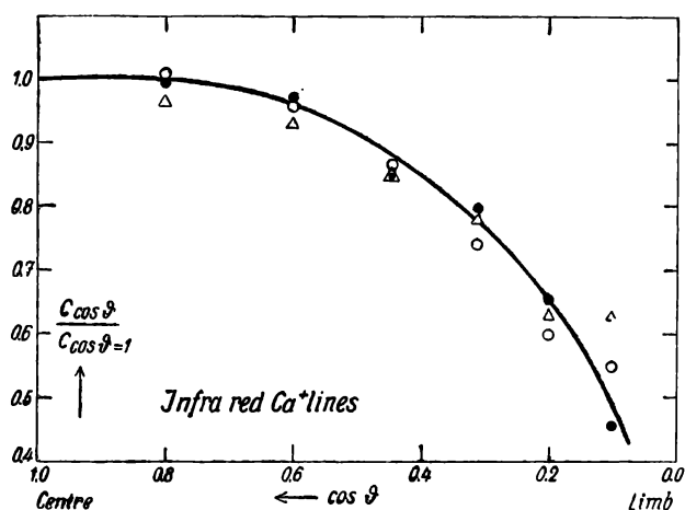
Fig. 33. — Centre-limb variations of the c 's of the infra-red \text{Ca}^+ lines; ● \text{Ca}^+ 8542.1 ; ○ \text{Ca}^+ 8662.2 ; △ \text{Ca}^+ 8498.0 .
