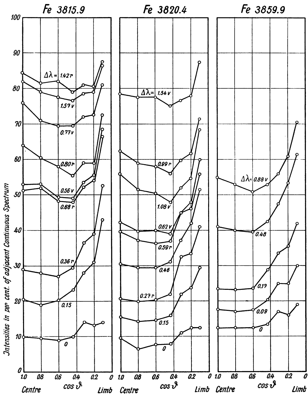
Fig. 4. — Centre-limb variations in the profiles of three ultra-violet Fe lines (parameter \Delta\lambda = distance in Å from centre of line).
