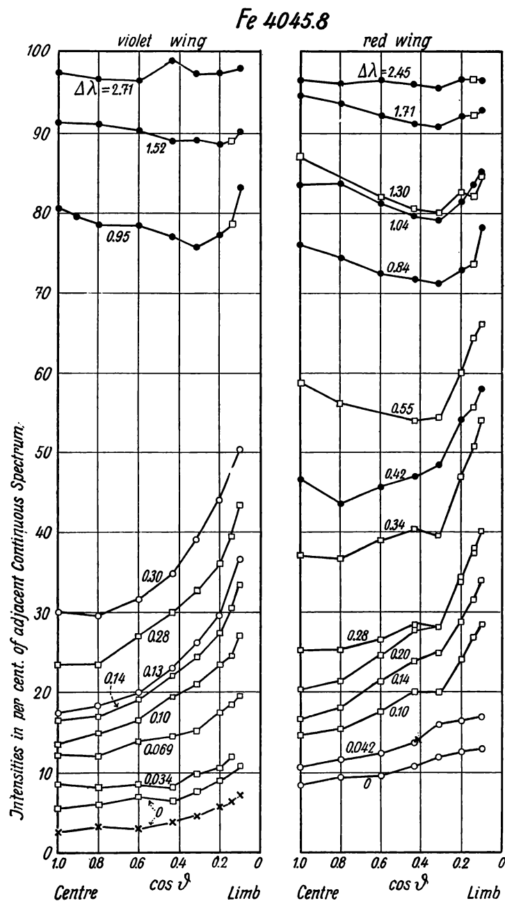
Fig. 12. — Centre-limb variations in the line Fe 4045.8; ○ Utrecht; □ Potsdam; ● mean; × corrected central intensities (parameter \Delta\lambda = distance in Å from centre of line).
