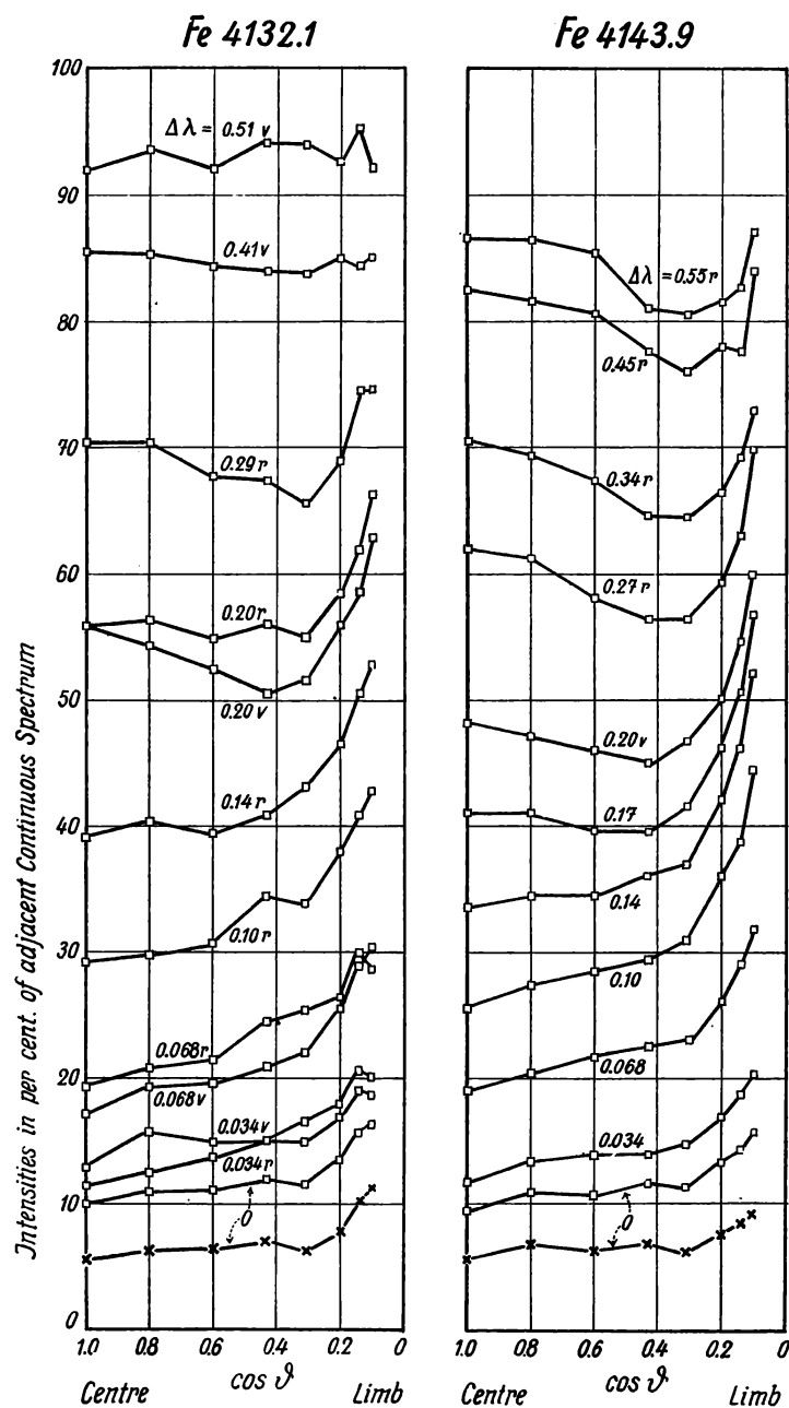
Fig. 18. — Centre-limb variations in the lines Fe 4132.1 and 4143.9; \times corrected central intensities (parameter \Delta\lambda = distance in Å from centre of line).
