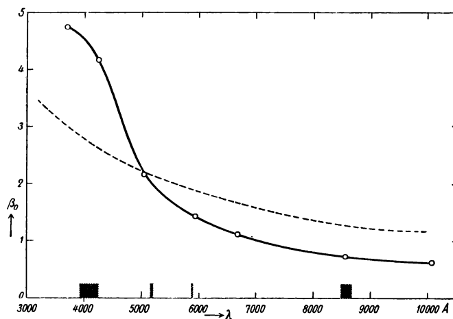
Fig. 38. — Run of \beta_0 with wave length; — deduced from C. G. Abbot's measurements of the darkening of the continuous spectrum towards the limb; — — — theoretical run in the case of local thermodynamical equilibrium and when \kappa(\lambda, \tau) = \text{constant} (A. Unsöld). Along the \lambda -axis are marked the locations of the measured Fraunhofer lines.
