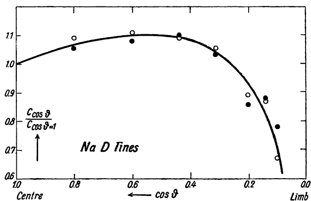
Fig. 30. — Centre-limb variations of the c 's of the D lines of Na; ● Na 5890.0; ○ Na 5895.9.
