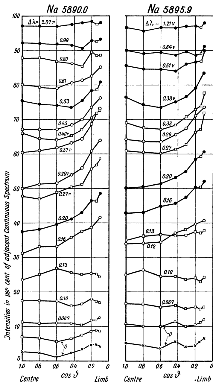
Fig. 27. — Centre-limb variations in the Na D lines; O Utrecht; □ Potsdam; ● mean; × corrected Potsdam central intensities (parameter \Delta\lambda = distance in \text{\AA} from centre of line).
