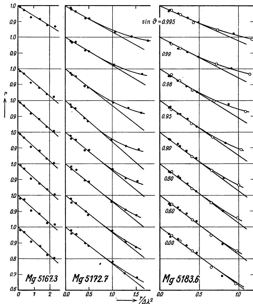
Fig. 24. — Determination of the c 's of the Mg b lines; the points \bigcirc are the means of 3 or 4 values from the intensity lists (Tables 13—15). The scales for the abscissae are chosen in such a way that, for equal values of \sin \theta , the slopes of the tangents would be the same for all three of the lines, if the c 's were to each other in the same ratio as the multiplet intensities.
