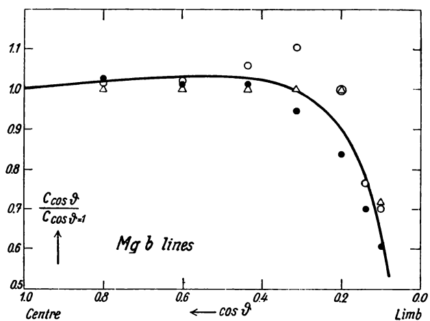
Fig. 26. — Centre-limb variations of the c 's of the Mg b lines; ● Mg 5183.6; ○ Mg 5172.7; △ Mg 5167.3.
