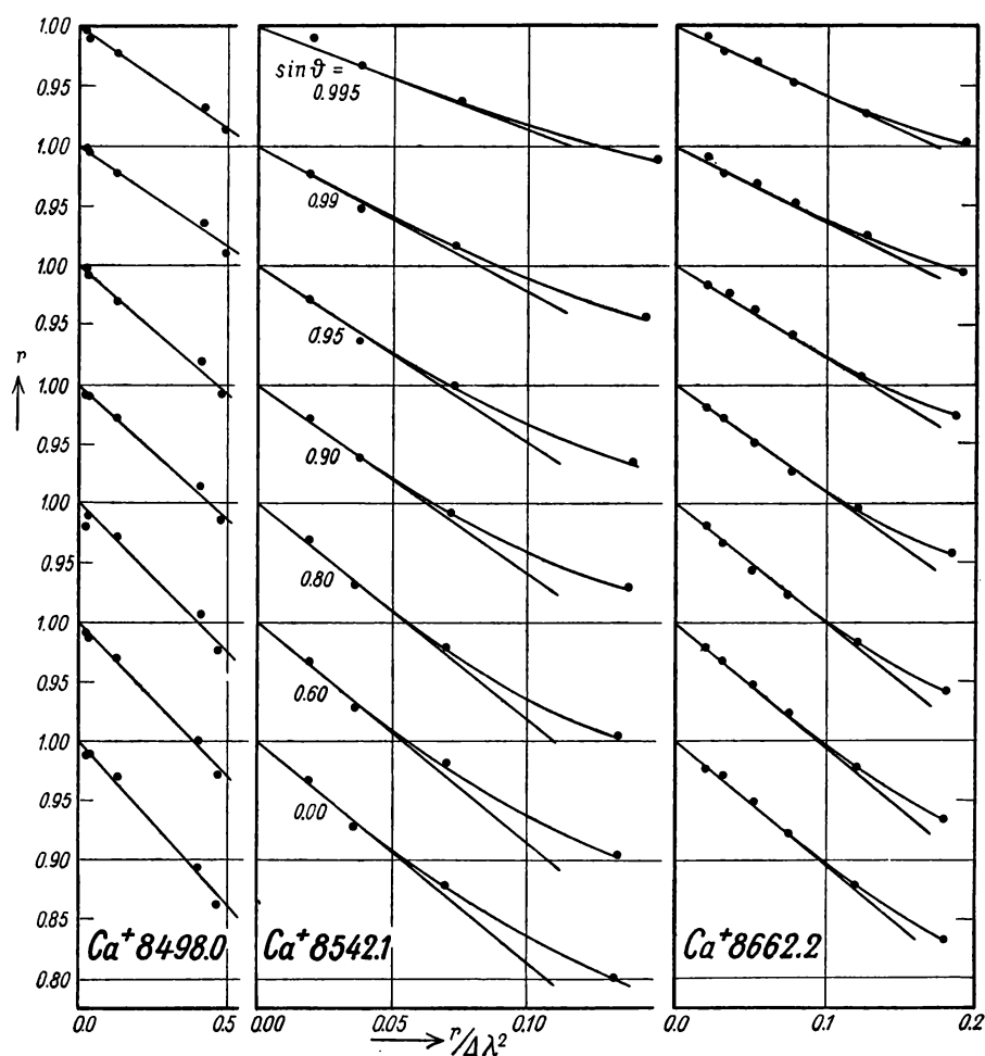
Fig. 34. — Determination of the c 's of the infra-red \text{Ca}^+ lines. The scales of the abscissae are chosen in such a way that, for equal values of \sin \vartheta , the slopes of the tangents would be the same for all three of the lines, if the c 's were to each other in the same ratio as the multiplet intensities.
