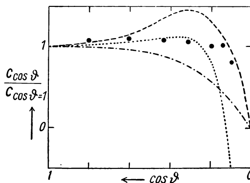
Fig. 46. — Centre-limb variations of the c 's for the Na D lines. Theoretical curves, for which the run of k and s is the same as that of Strömgren's \eta in the far wings (see Fig. 43): — . — absorption and coherent scattering with B = B_0(1 + 1.69\tau) ; ---- absorption, ..... coherent scattering, both with B according to Plaskett (c.f. Fig. 45). ● From observations.
