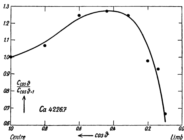
Fig. 21. — Centre-limb variation of the c 's of the line Ca 4226.7.
