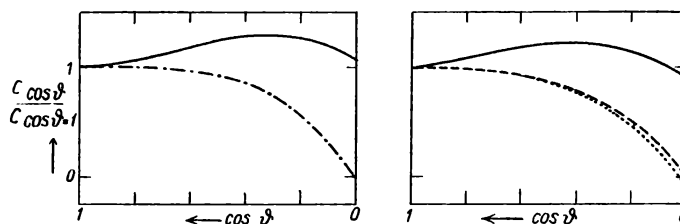
Fig. 44. — Centre-limb variations of the c 's for the Na D lines. Left: computed with a run of k , s and l which is the same as that of Strömgren's \eta (using run for wing of Fig. 43). Right: k , s and l according to our simple model with \tau_1 = 1.5 , computed with formula (21) (c.f. Fig. 43).
