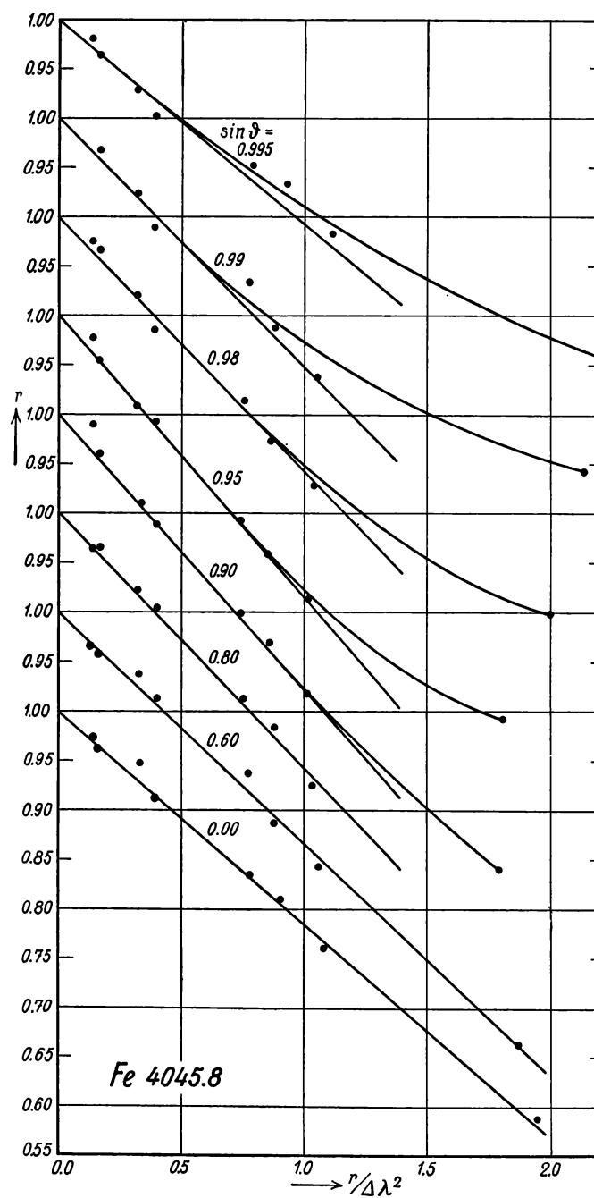
Fig. 13. — Determination of the c 's of the line Fe 4045.8.
