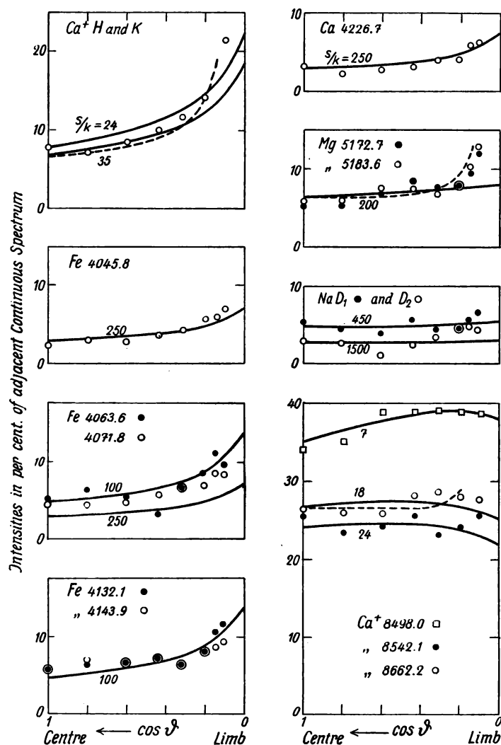
Fig. 49. — Centre-limb variations of the central intensities; — computed with the aid of formula (48); the values of s/k belong to these curves; — — — computed with the numerator of (48) and the darkening of the continuous spectrum towards the limb, according to the observations by W. J. H. Moll, H. C. Burger and J. v. d. Bilt; these curves have been made to coincide for \cos \vartheta = 1 with one of the curves computed from (48); for lines located in the same spectral region the ratios between the ordinates of — and — — — are the same for corresponding \cos \vartheta .
