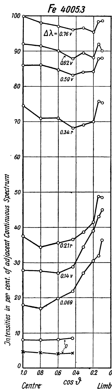
Fig. 11. — Centre-limb variations in the line Fe 4005.3 (parameter \Delta\lambda = distance in Å from centre of line); X corrected central intensities.
