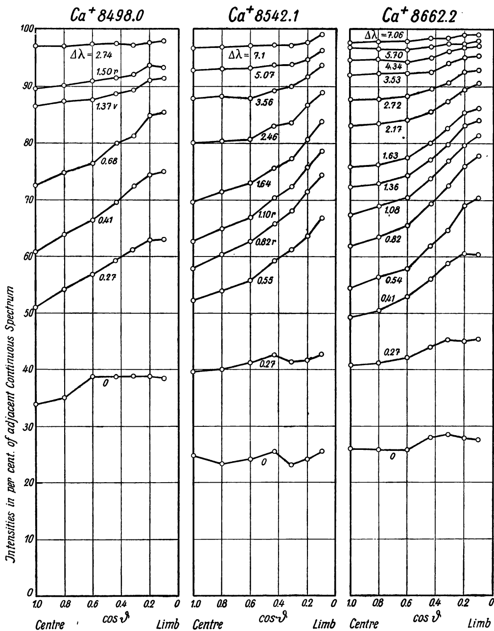
Fig. 31. — Centre-limb variations in the lines \text{Ca}^+ 8498.0 , \text{Ca}^+ 8542.1 and \text{Ca}^+ 8662.2 ; (parameter \Delta\lambda = distance in Å from centre of line).
