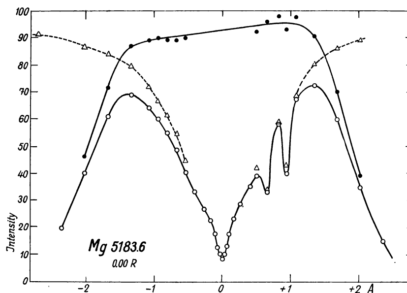
Fig. 1. — Determination of the inner part of the profile of a strong Fraunhofer line; exposure with narrow monochromator-slit in order to avoid scattered light and ghosts (first ghost at 3.5 Å from principal line);
