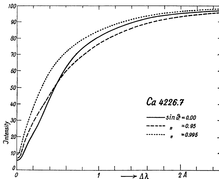
Fig. 20. — Profiles of the line Ca 4226.7 in three different points of the solar disc (non-corrected central intensities).
