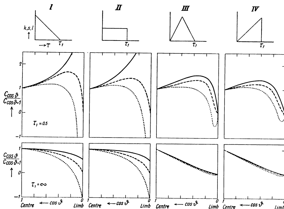
Fig. 42. — Computed centre-limb variation of c for various cases of the run with depth of k, s and l , all of them for \beta_0 = 4.5 (violet part of the spectrum): — — — absorption, ..... coherent scattering, — — — extinction. As appears from the drawings at the top, the four models are arranged according to decreasing concentration at the surface; in each of the models \tau_1 can vary from 0 - \infty , from this range the values 0.5 and \infty have been selected for the construction of the figures.
