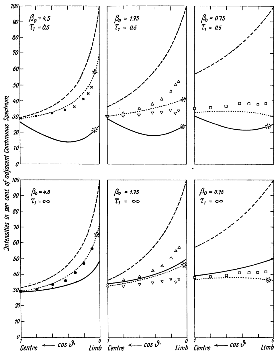
Fig. 48. — Centre-limb variations in the Fraunhofer lines. Theoretical curves: ——— absorption, ..... coherent scattering, ——— extinction. Observations: ● H- and K line of Ca + , × Fe multiplet and Ca 4226.7, △ Mg b lines, ▽ Na D lines, □ infra-red lines of Ca + . The theoretical curves, appropriate to a comparison with the observations, are marked with an asterisk (extinction is only to be expected in a comparatively thin surface-layer); the comparison concerns the centre-limb variations; the heights of the various theoretical curves and of the observational points are, therefore, adapted as well as possible to each other.
