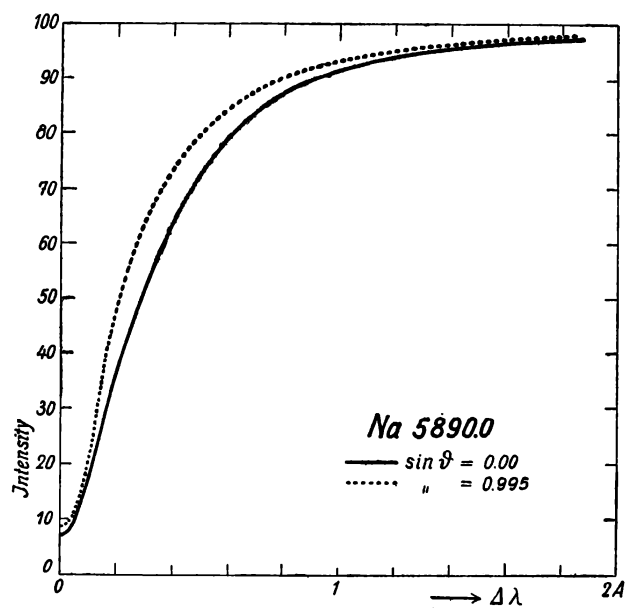
Fig. 29. — Profiles of the D 2 line of Na in two different points of the solar disc (non-corrected central intensities).
