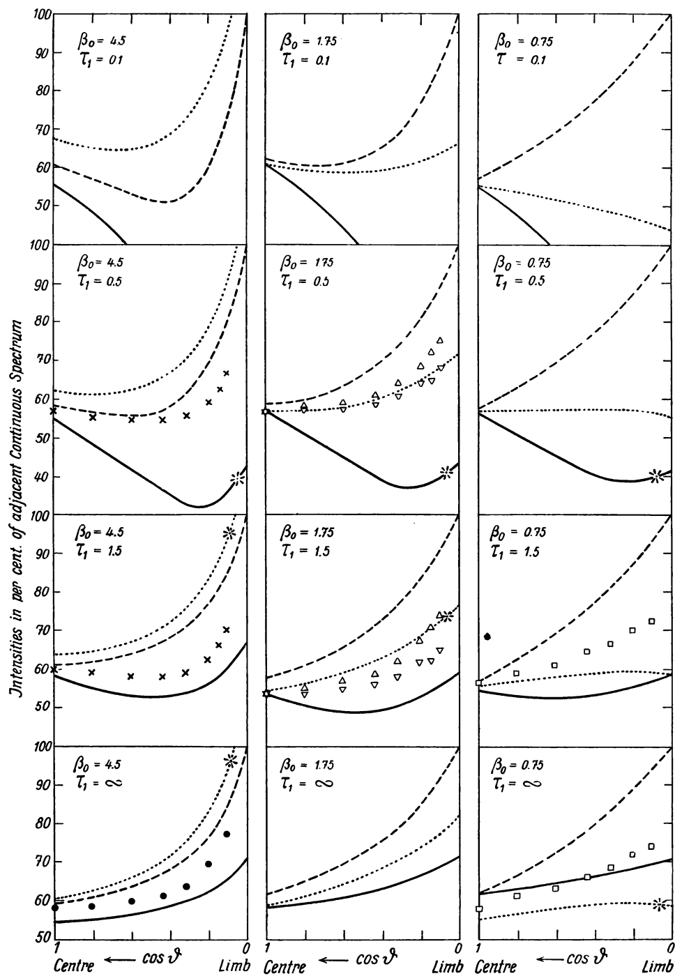
Fig. 47. — Centre-limb variations in the wings of the Fraunhofer lines. Theoretical curves: — — — absorption, ..... coherent scattering, — — — extinction. Observations: ● H- and K line of Ca + , × Fe multiplet and Ca 4226.7, △ Mg b lines, ▽ Na D lines, □ infra-red lines of Ca + . For further explanations see Fig. 48.
