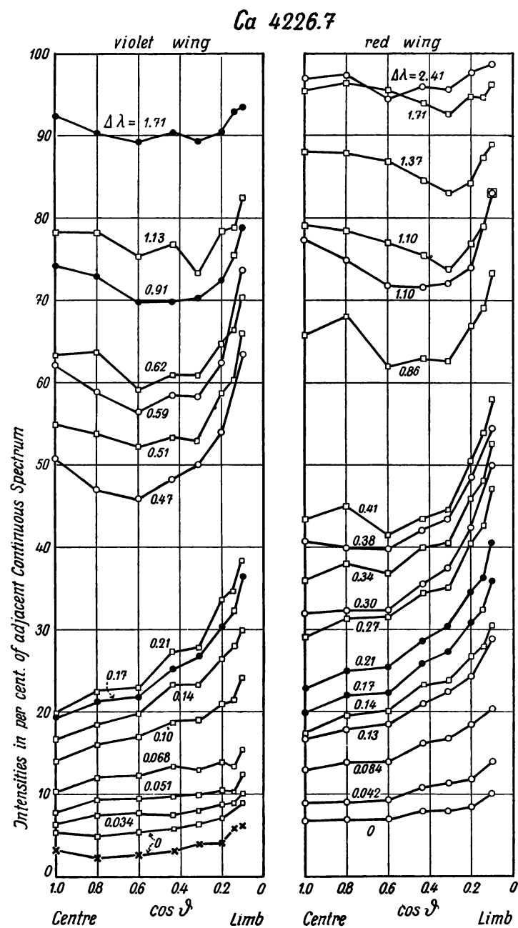
Fig. 22. — Centre-limb variations in the line Ca 4226.7; ○ Utrecht; □ Potsdam; ● mean; × corrected central intensities (parameter \Delta\lambda = distance in Å from centre of line).
