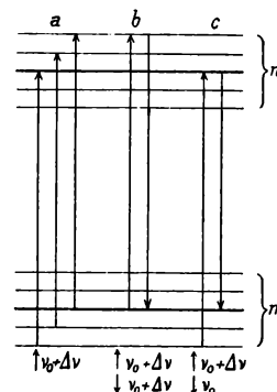
Fig. 37. Widened energy-levels; when radiation of frequency \nu_0 + \Delta\nu is absorbed, maxima of emission occur at frequencies \nu_0 + \Delta\nu and \nu_0 .
