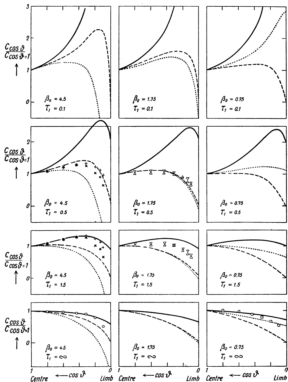
Fig. 41. — Computed centre-limb variations of c : ——— absorption, ..... coherent scattering, ——— extinction. Observations added: \circ K line of \text{Ca}^+ , + Fe multiplet at 4100 Å, \times Ca 4226.7, \triangle Mg b lines, \triangle Na D lines, \square infra-red lines of \text{Ca}^+ .
