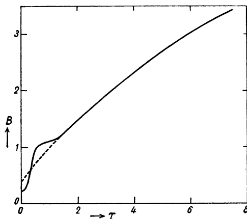
Fig. 45. — Run of B , computed by H. H. Plaskett from the observations of W. J. H. Moll, H. C. Burger and J. v. d. Bilt; ---- J , the radiation-density in the far wings of a Fraunhofer line.
