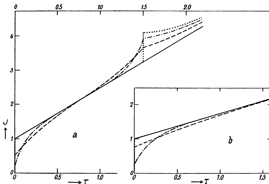
Fig. 40. — Runs of B and J(s) with depth in the schematic model of the solar atmosphere. a) \beta_0 = 1.5 , \tau_1 = 1.5 ; ——— B and J(s=0) , — — — J(s=3) , — · — J(s=29) , · · · J(s=\infty) . b) \beta_0 = 0.75 , \tau_1 = \infty ; ——— B , — — — J(s=0) , — · — J(s=10) , · · · J(s=\infty) .
