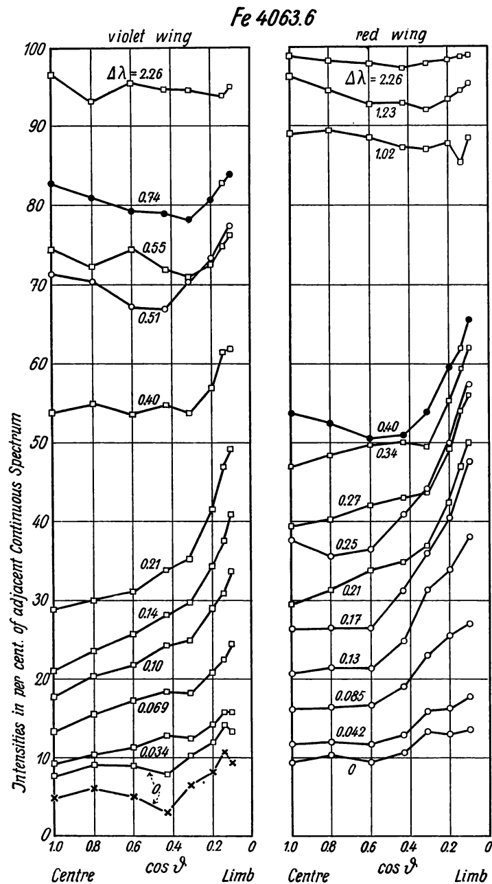
Fig. 16. — Centre-limb variations in the line Fe 4063.6; ○ Utrecht; □ Potsdam; ● mean; × corrected central intensities (parameter \Delta\lambda = distance in Å from centre of line).
