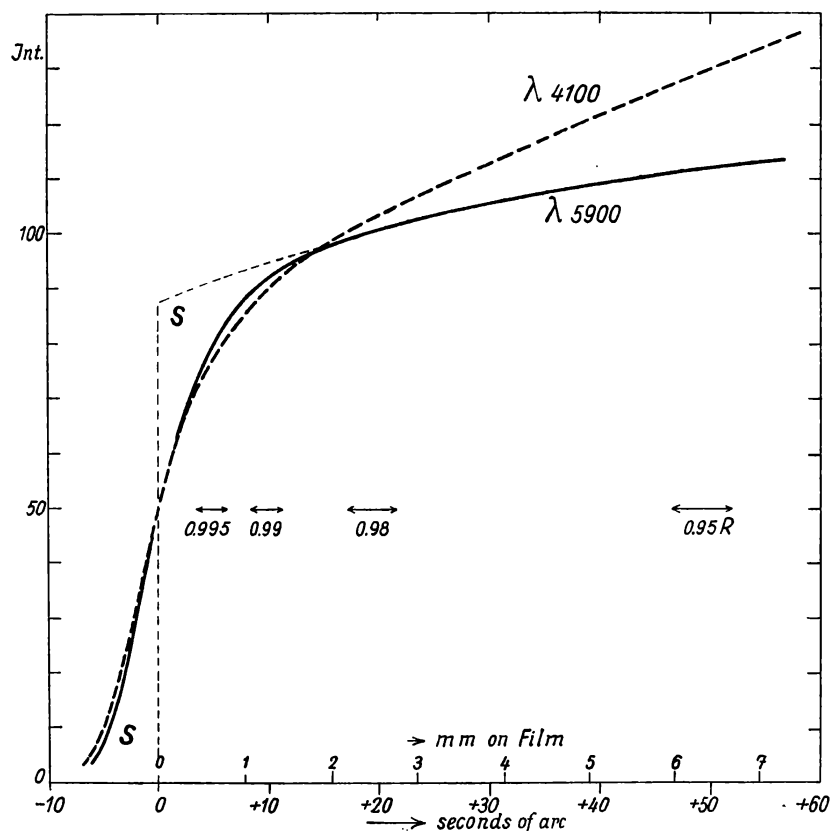
Fig. 2. — Intensity of the continuous background along a radius of the solar disc near the sun's limb; at \lambda 4100 from photographs of the Fe multiplet and at \lambda 5900 from the Na D doublet. The double arrows indicate the places used in registering the spectra, while their lengths correspond to the lengths of the photometer-slit. The abscissa of the sun's limb is fixed by the condition that the areas S shall be equal.
