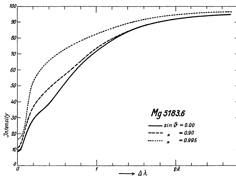
Fig. 25. — Profiles of the line Mg 5183.6 in three different points of the solar disc (non-corrected central intensities).
