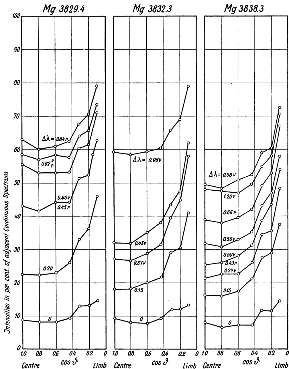
Fig. 5. — Centre-limb variations in the profiles of three ultra-violet Mg lines (parameter \Delta\lambda = distance in Å from centre of line).
