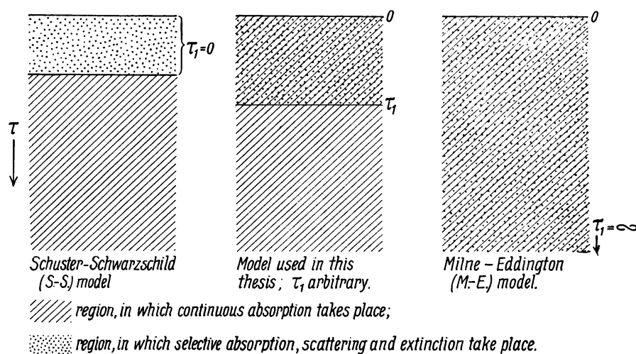
Fig. 35. — Three schematic models of the solar atmosphere.
