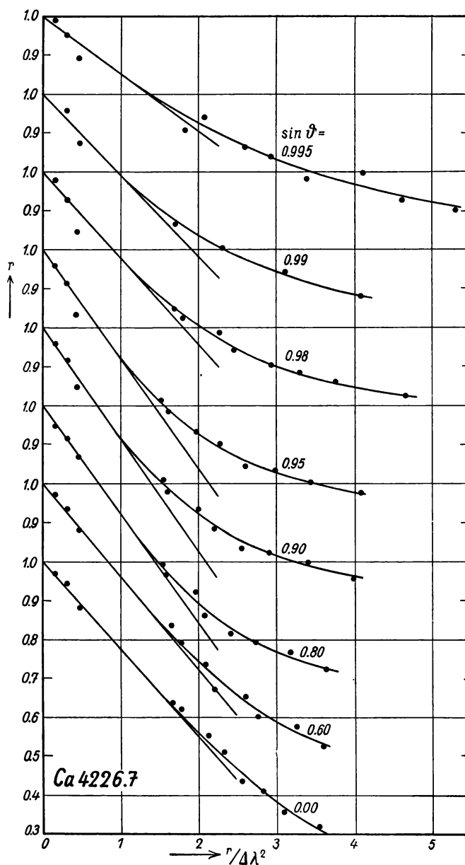
Fig. 19. — Determination of the c 's of the line Ca 4226.7.
