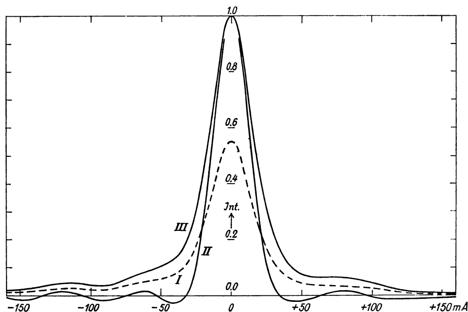
Fig. 3. — I: instrumental curve of the Potsdam grating spectrograph for \lambda 5000; II: instrumental curve I transformed by the peak-function operation; I and II have equal areas; III: instrumental curve obtained from I by multiplying its ordinates so that the top coincides with that of II.
